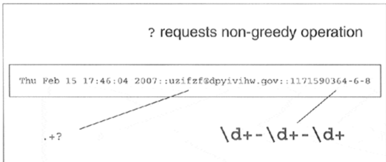
Figure 15.3. Solving the Greedy Problem: ? Requests Non-Greediness
