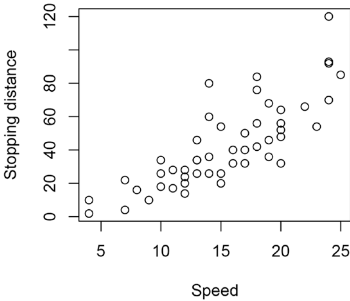
Figure 4-2. A scatterplot of speed and distance for cars
