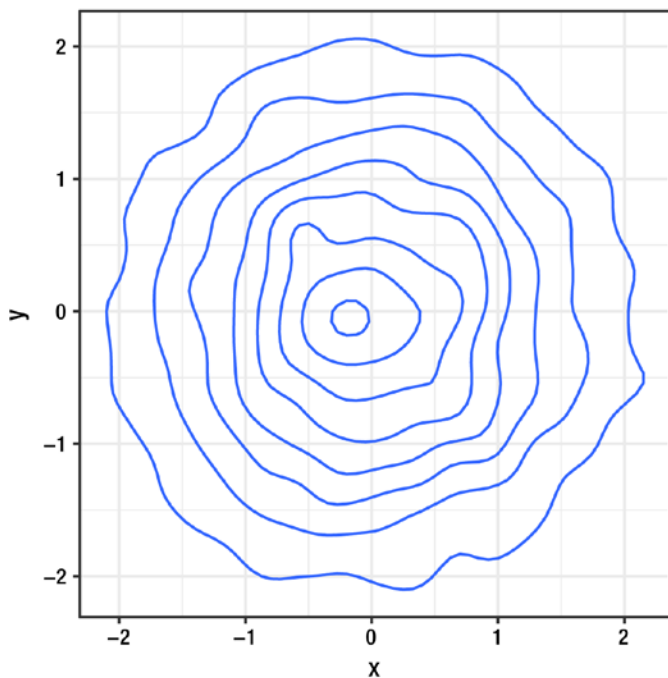
Figure 5-3. A 2D density plot
