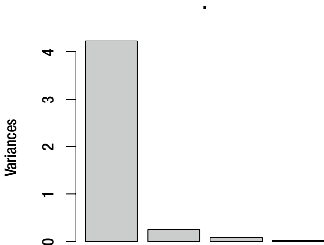
Figure 7-3. Plot of the variance on each principal component for the iris dataset
