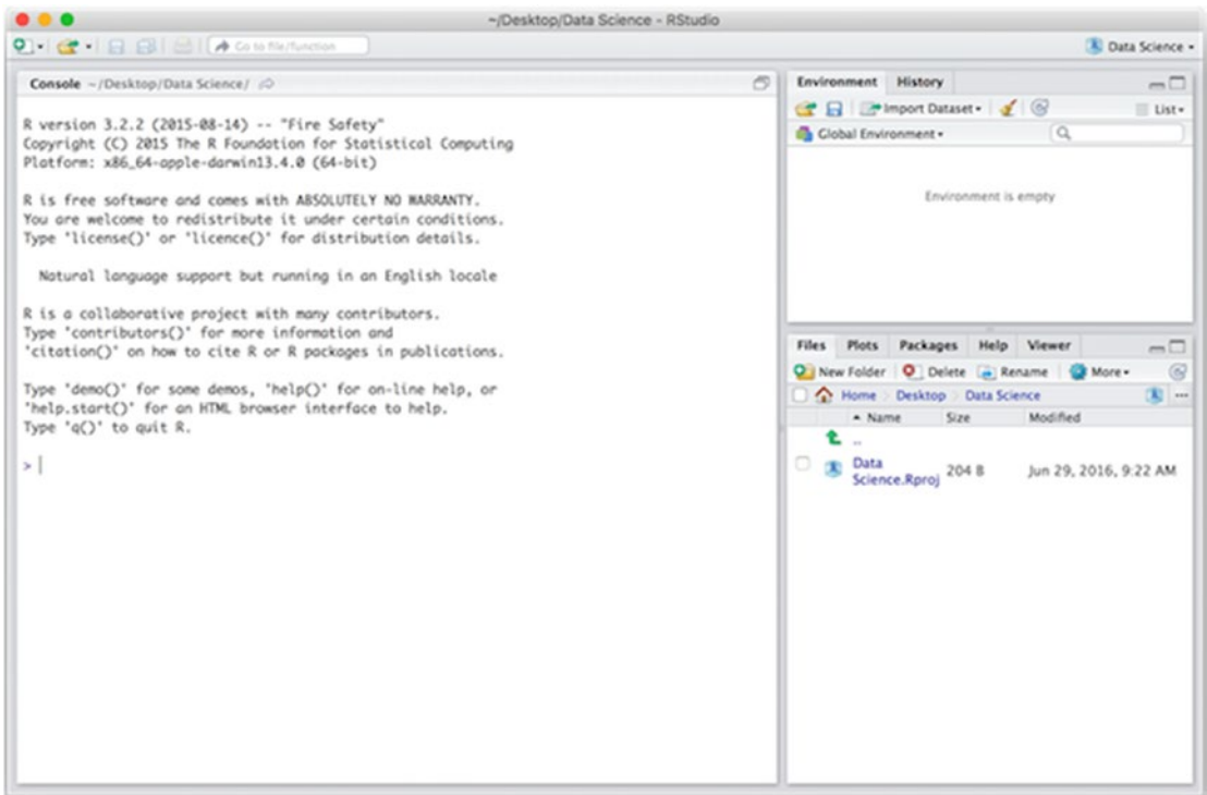
Figure 1-1. RStudio
