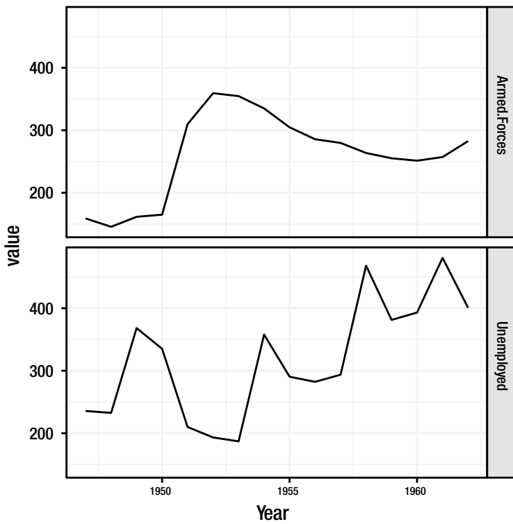
Figure 4-20. Longley data plotted using facets
