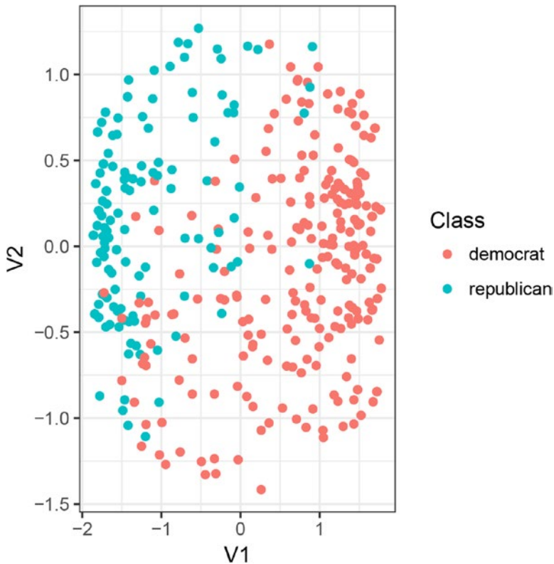
Figure 7-7. Multidimensional scaling plot for house voting data
