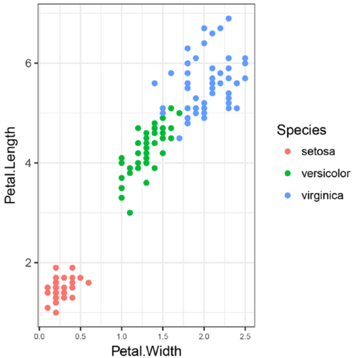
Figure 4-10. Plot of iris data with colors determined by the species. Plotted with qplot ( ggplot2 ).
