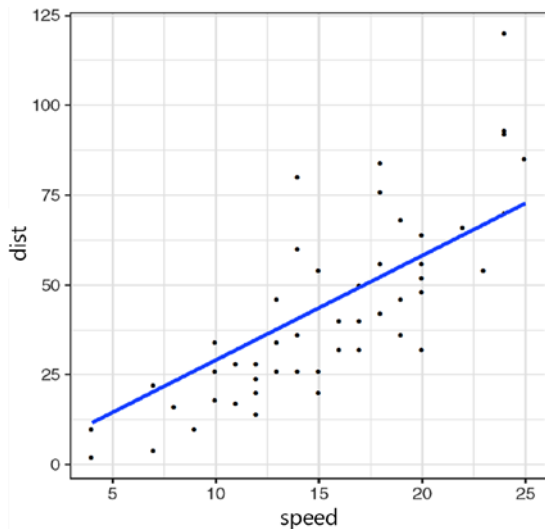
Figure 6-4. Best regression line going through (0,0)
