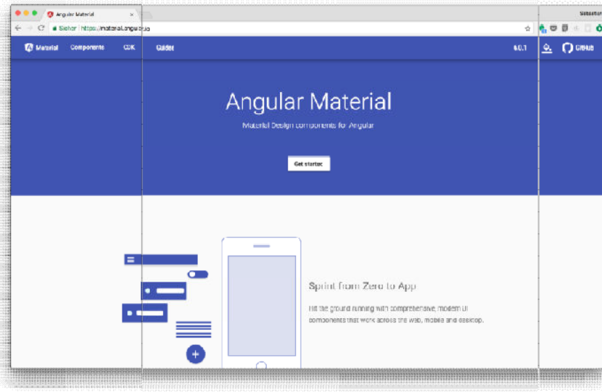
Fig 1.11 Angular Material
