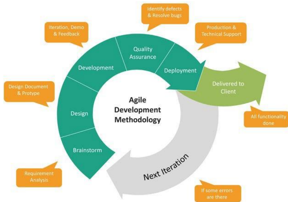
Fig 3.1 Agile Methodology
