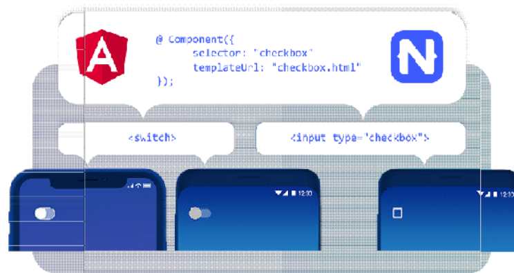
Fig 1.4 : Angular + NativeScript
