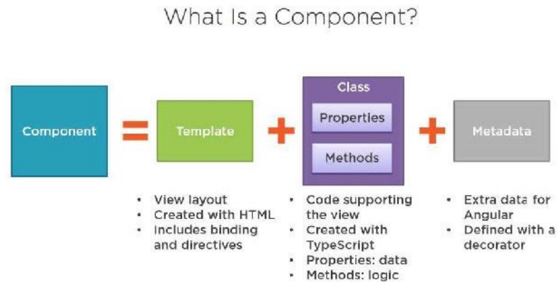
Fig 4.4: Angular Component
