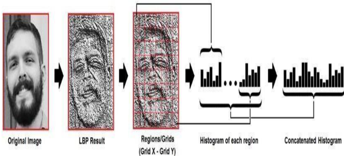
Figure 4.10: LBP result
