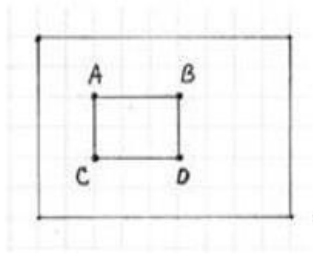
Figure 3.1: Recatangle used
