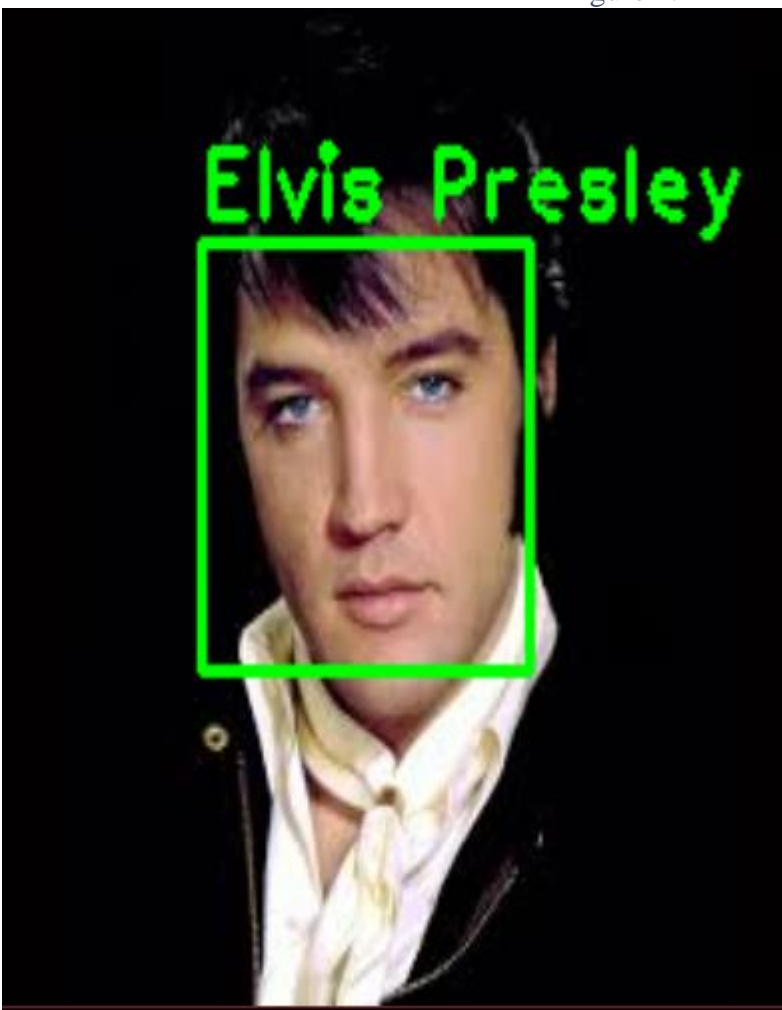
Figure 4.15
