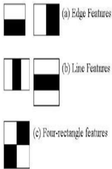
Figure 3.3
