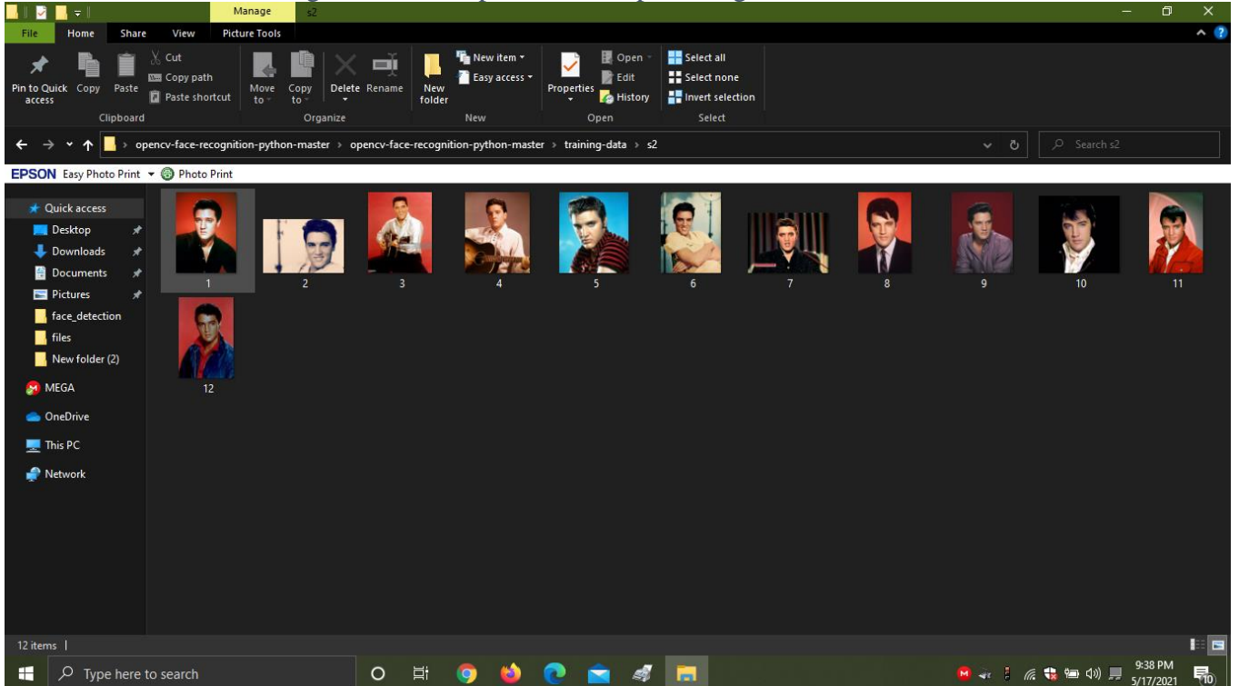
Figure 4.4: Another example
