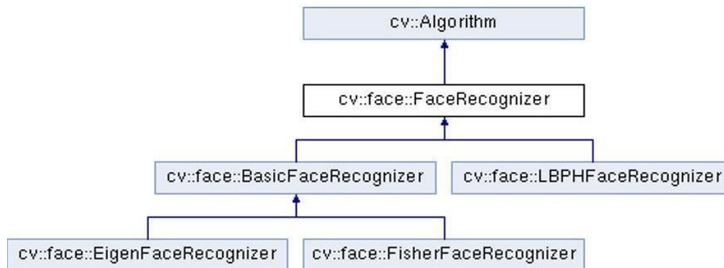
Figure 4.8: Flowchart Representaton
