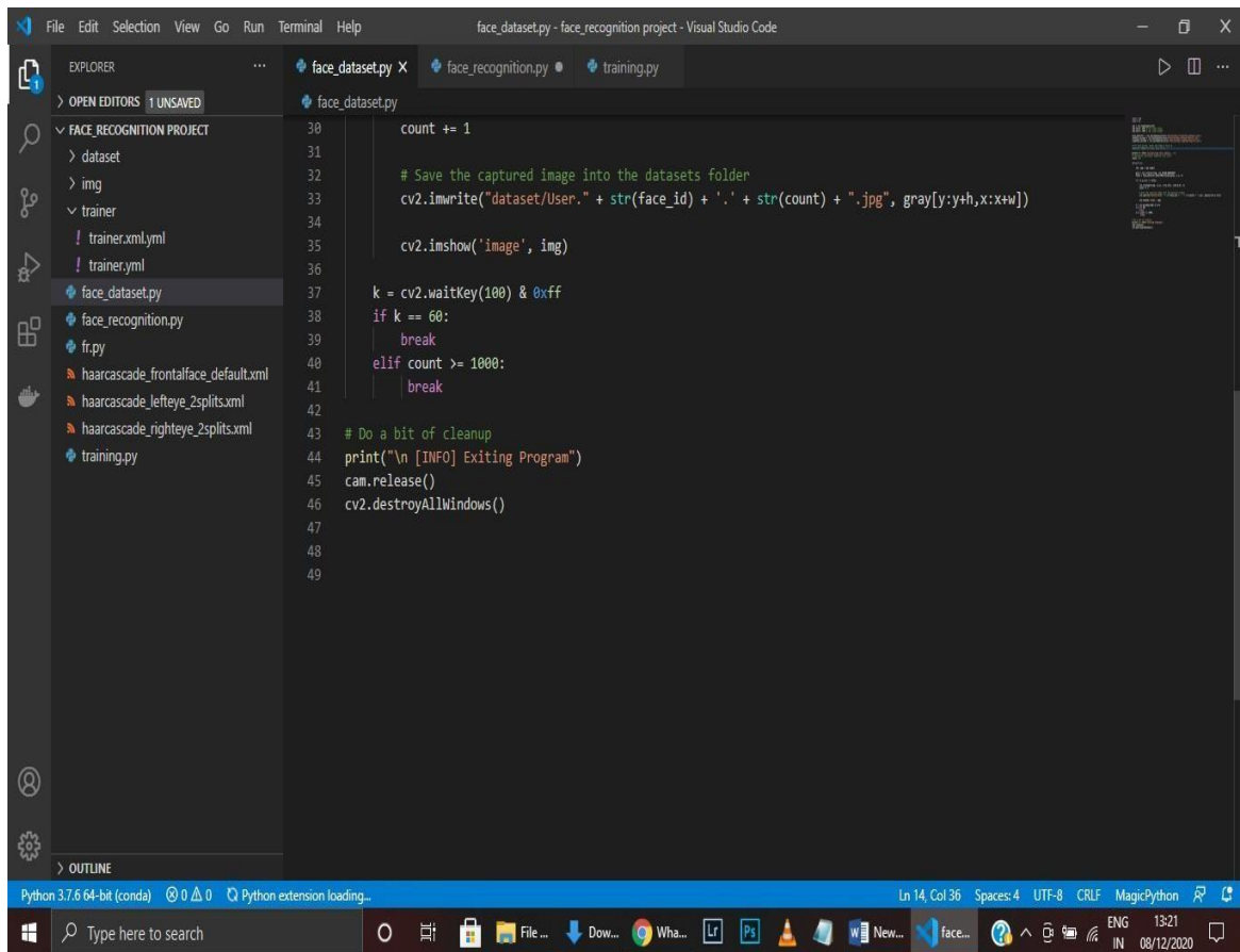
Figure 4.2: Face_dataset.py
