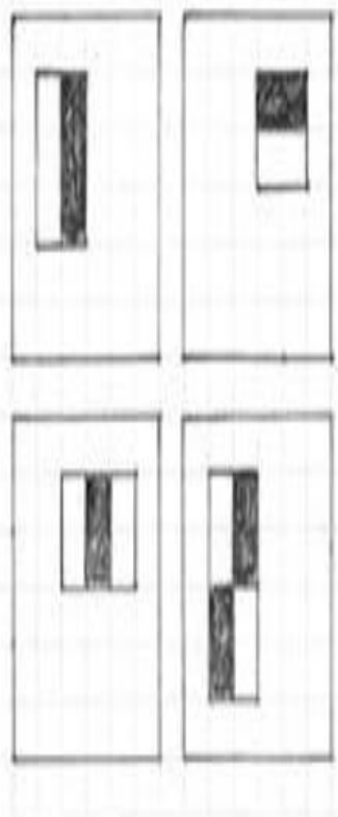
Figure 3.2:Classifiers
