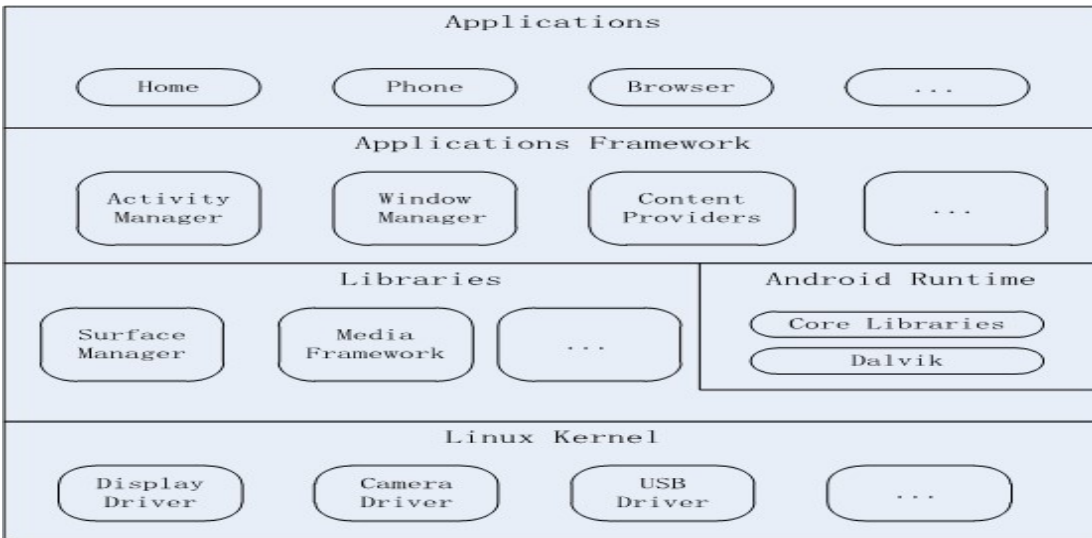
Figure2. Android Architecture
