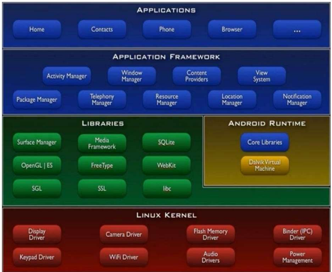
Figure 7. Android Architecture
