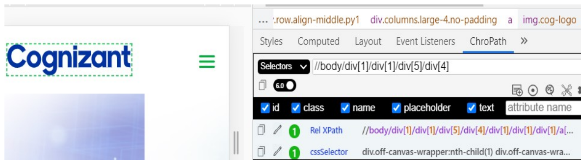
Figure 4.3: XPATH Example
