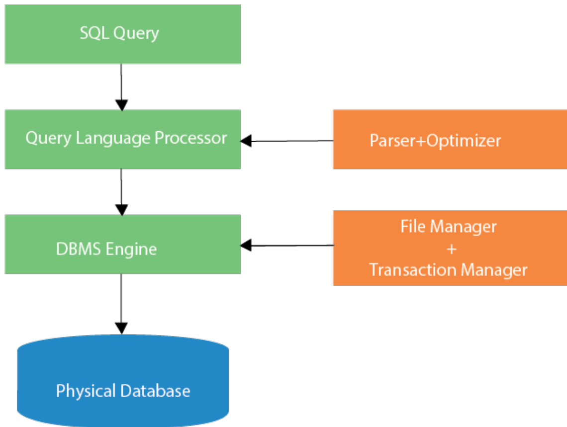
Figure 4.5: SQL architecture
