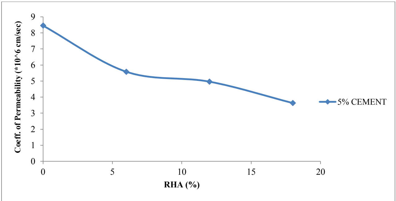
Figure 4.29 : Graph showing Coefficient of Permeability (k) for Different proportions of RHA at 5% Cement mix
