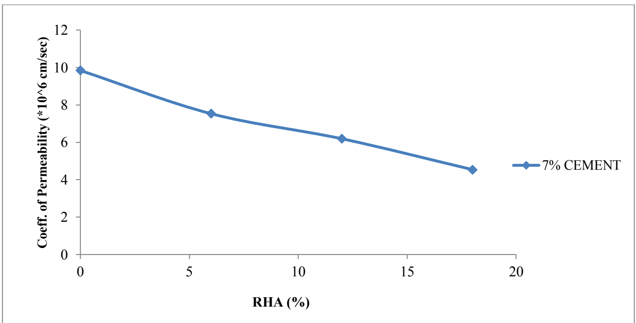
Figure 4.30 : Graph showing Coefficient of Permeability (k) for Different proportions of RHA at 7% Cement mix
