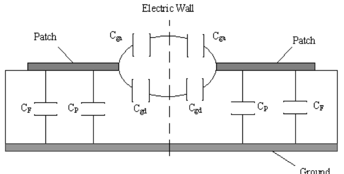
Figure 5: Odd-mode capacitances of the two gap-coupled circular microstrip patch antennas.
