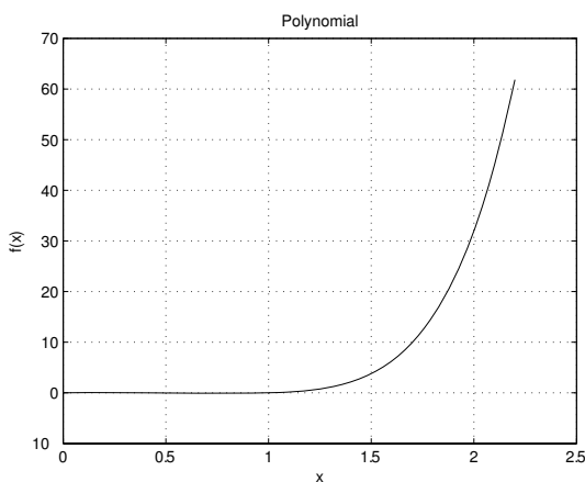
Fig. 8. Polynomial x^5(x - 0.7071)
