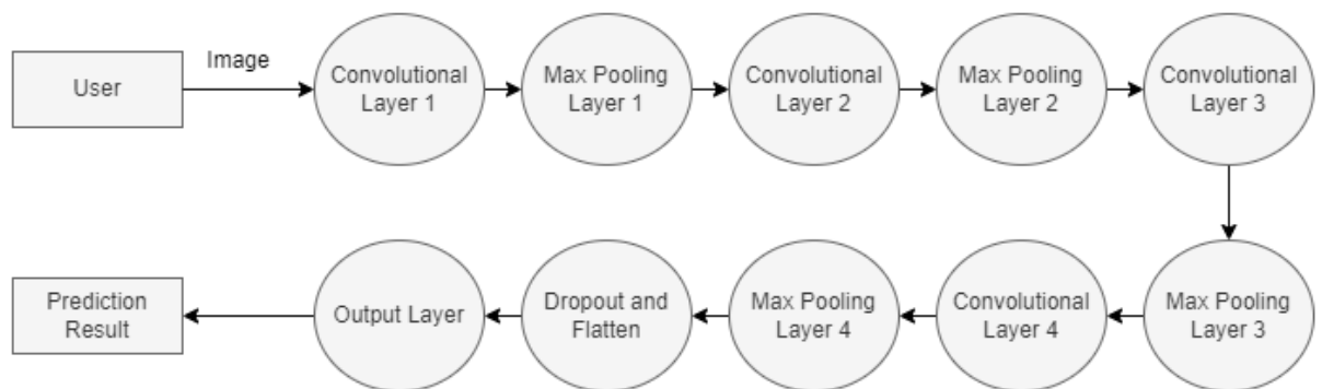
Fig 3.4: DFD Level 2
